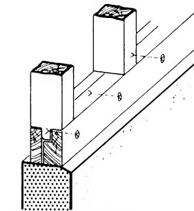
4 Sill replacement in two operations
